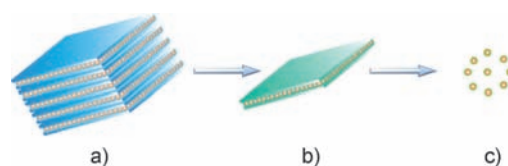
Figure 1. Disassembly of nanocluster-amine bilayer aggregates.
